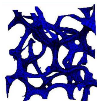
FE mesh of the foam using tetrahedral elements
