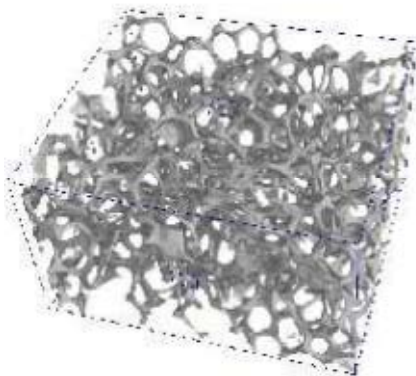
CT scan of an ERG foam
